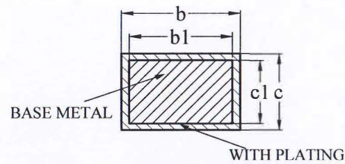
SECTION B-B
